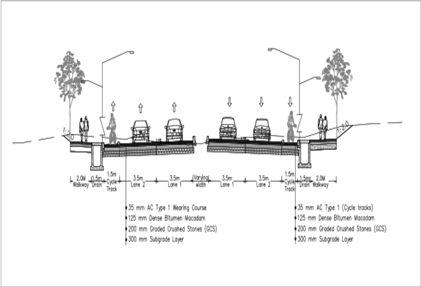
FIGURE 1: TYPICAL CROSS SECTION
