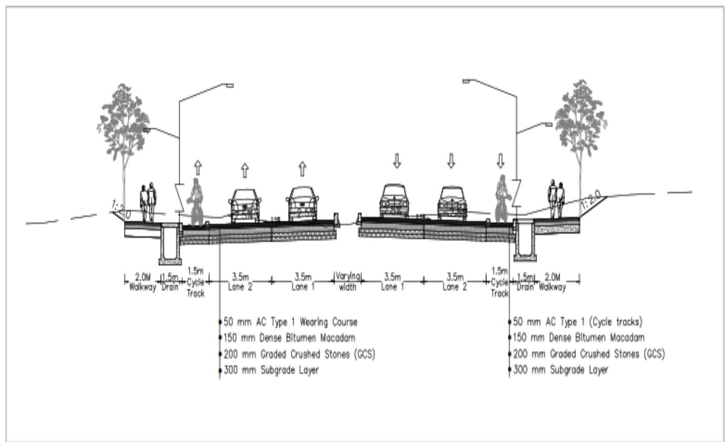
FIGURE 1: TYPICAL CROSS SECTION
