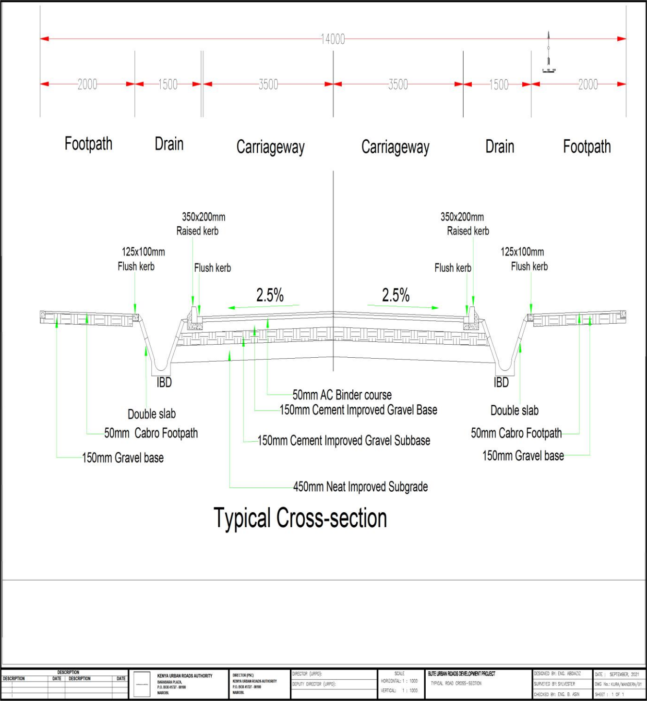
FIGURE 1: TYPICAL CROSS SECTION
