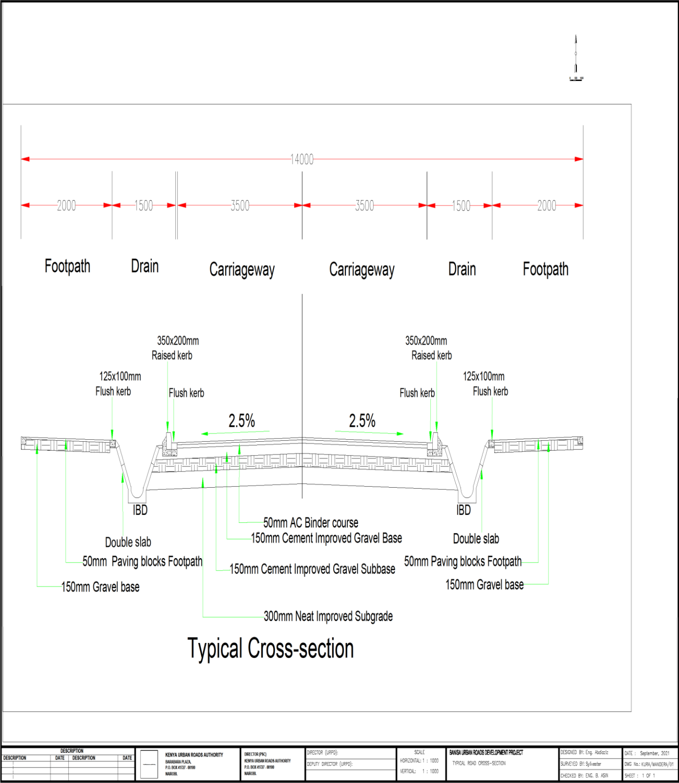
FIGURE 1: TYPICAL CROSS SECTION
