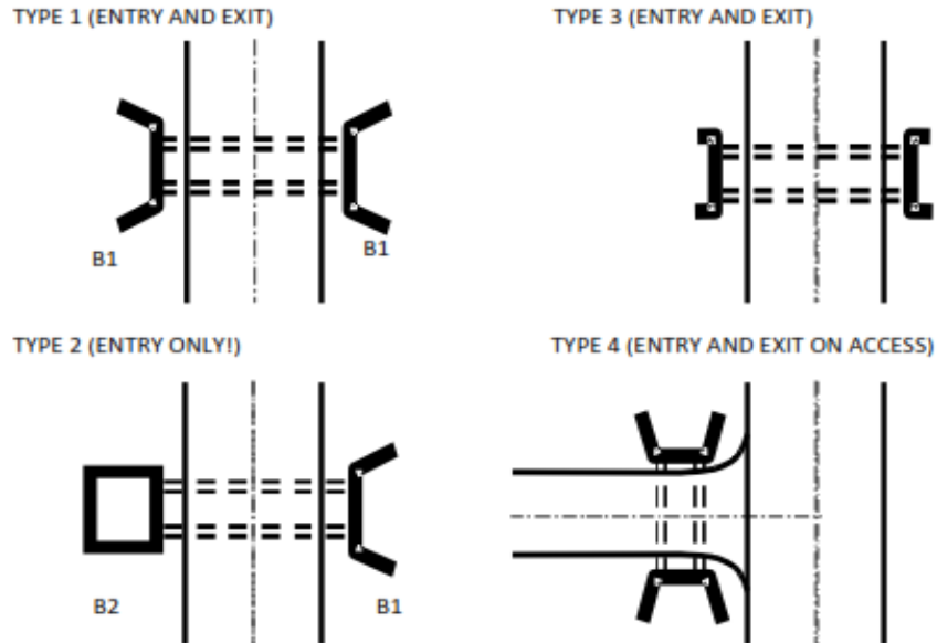
FIGURE C.1 - CULVERT ENTRY / EXIT STRUCTURE TYPES
